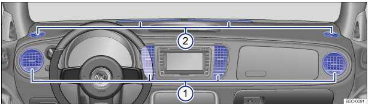
Fig. 110 In the instrument panel: Air vents.
